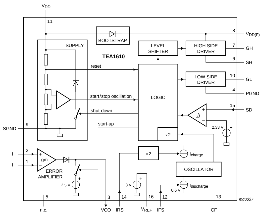
Fig 2. Block diagram
